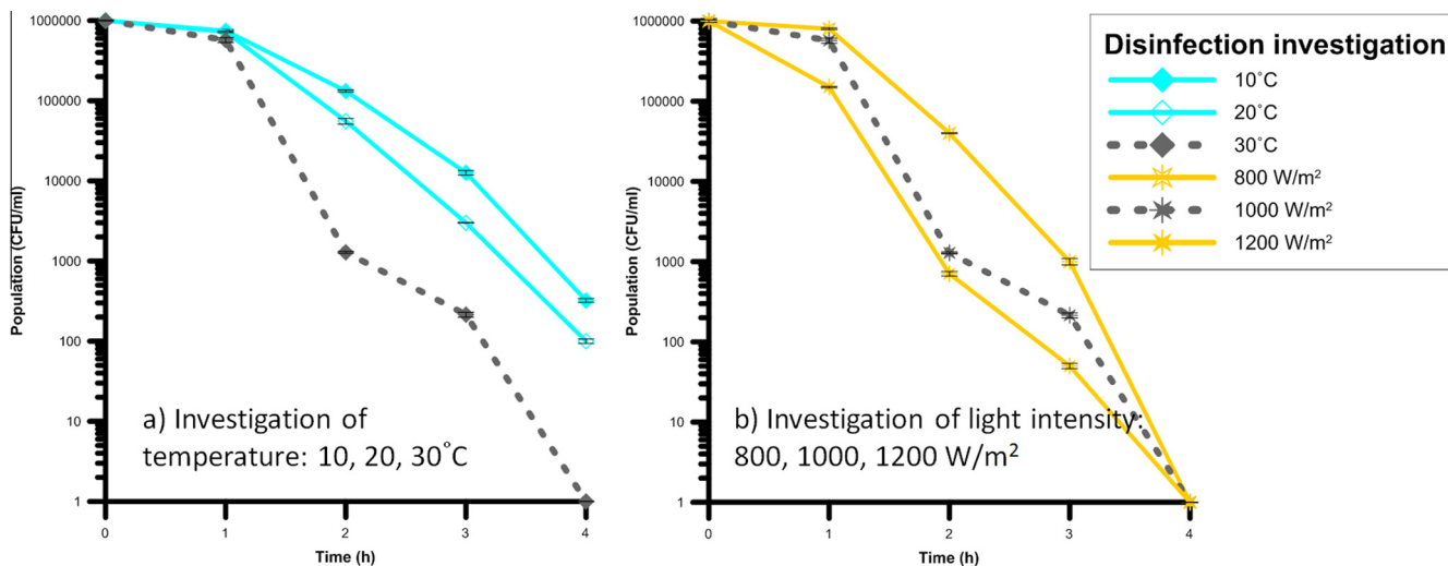
Fig. 5. Influence of the environmental parameters on the efficiency of the system. (a) Investigation of temperature (10, 20 and 30 °C), (b) Investigation of light intensity (800, 1000 and 1200 W/m 2 ).
