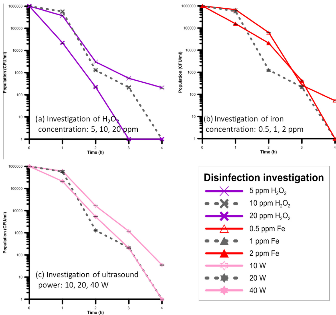
Fig. 6. Influence of the Fenton reagents and the sonication intensity on the efficiency of the system. (a) Investigation of the H 2 O 2 concentration (5, 10 and 20 ppm), (b) Investigation of the iron concentration (0.5, 1 and 2 ppm) and (c) Investigation on the ultrasound power (10, 20 and 40 W).
