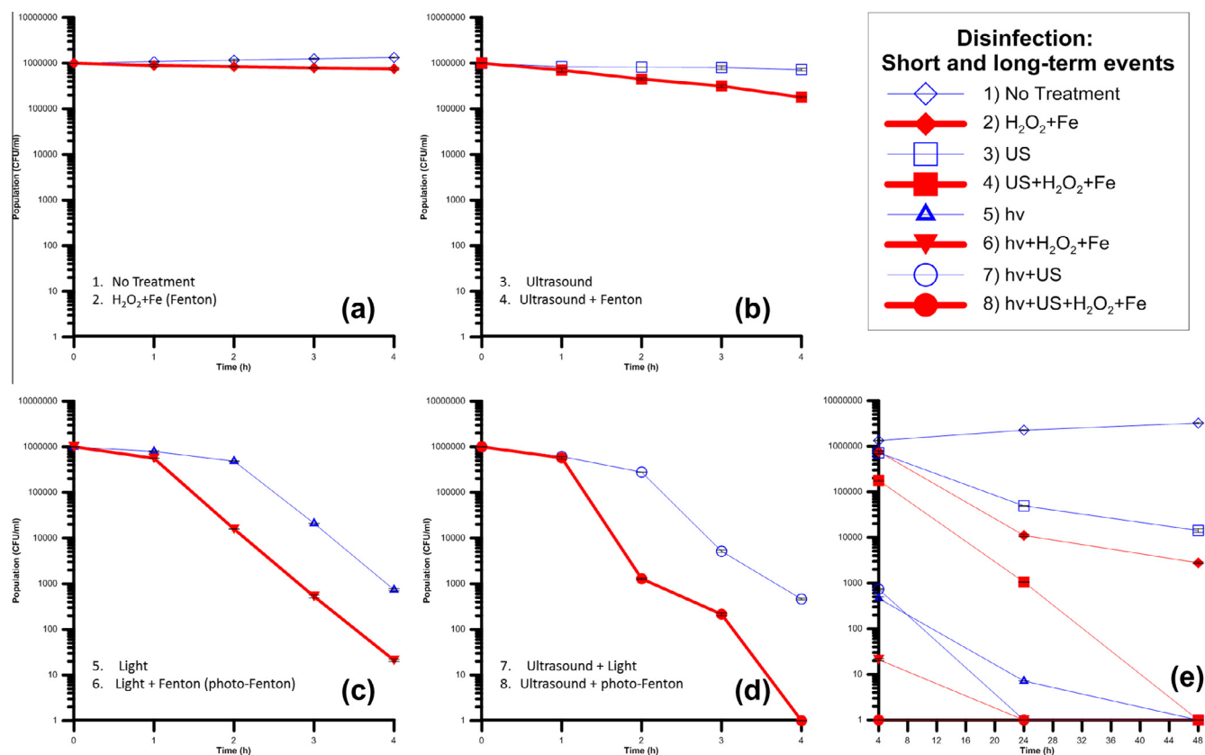
Fig. 2. Experimental results from the coupling of photo-Fenton and sonication. (a) Experiments 1–2 (WW and WW/Fe/H 2 O 2 ), (b) Experiments 3–4 (US and US/Fe/H 2 O 2 ), (c) Experiments 5–6 (hv and hv/Fe/H 2 O 2 ) and (d) Experiments 7–8 (hv/US and hv/US/Fe/H 2 O 2 ). (e) Long-term inactivation events for 48 h (time axis initiates in the 4-h mark, after treatment).
