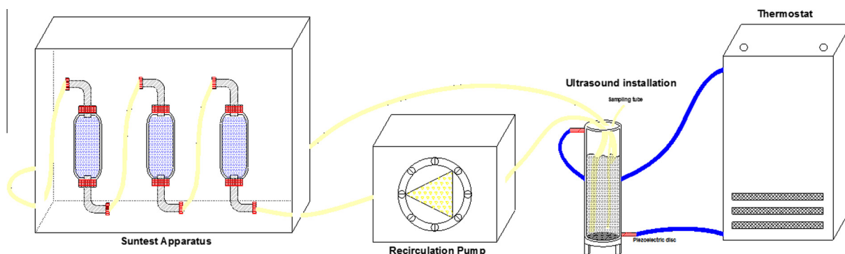
Fig. 1. Experimental set-up, consisting of the illuminated area (Suntest apparatus), the recirculation pump, the (dark) sonication vessel and the temperature control (thermostat). The flow direction is clockwise, water is introduced at surface level and sampled from the bottom of the vessel.
